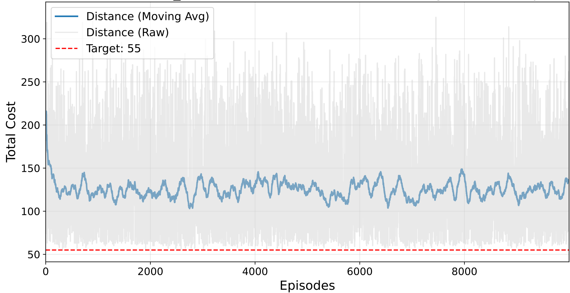
Final RANDOM_SEARCH Masked AutoRL-SOP Training - br17.10.sop
